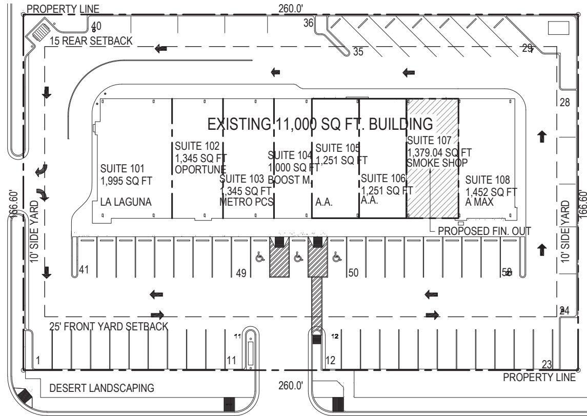
1 SITE PLAN NO SCALE
