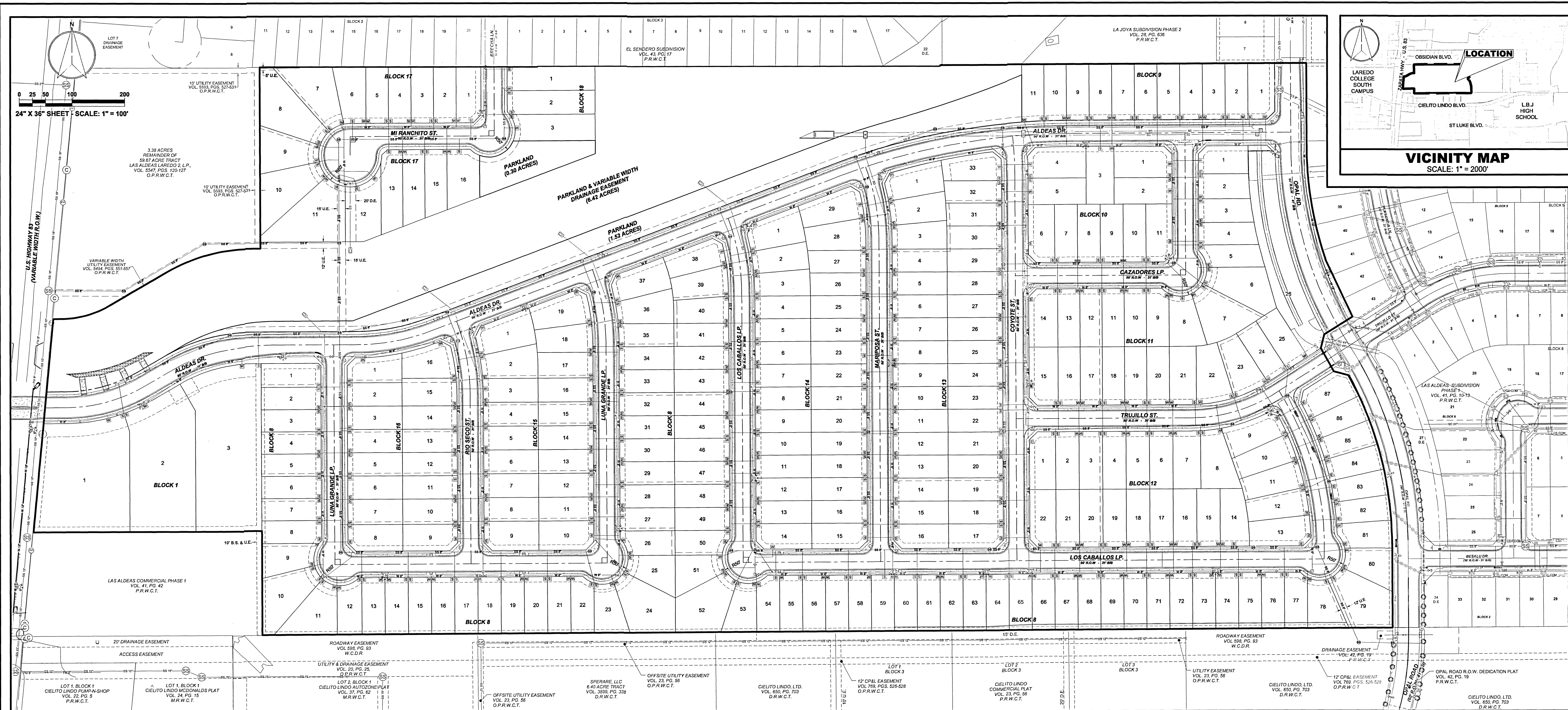
1 WATER DISTRIBUTION SYSTEM AND SANITARY SEWER SYSTEM SCALE: 1:100
