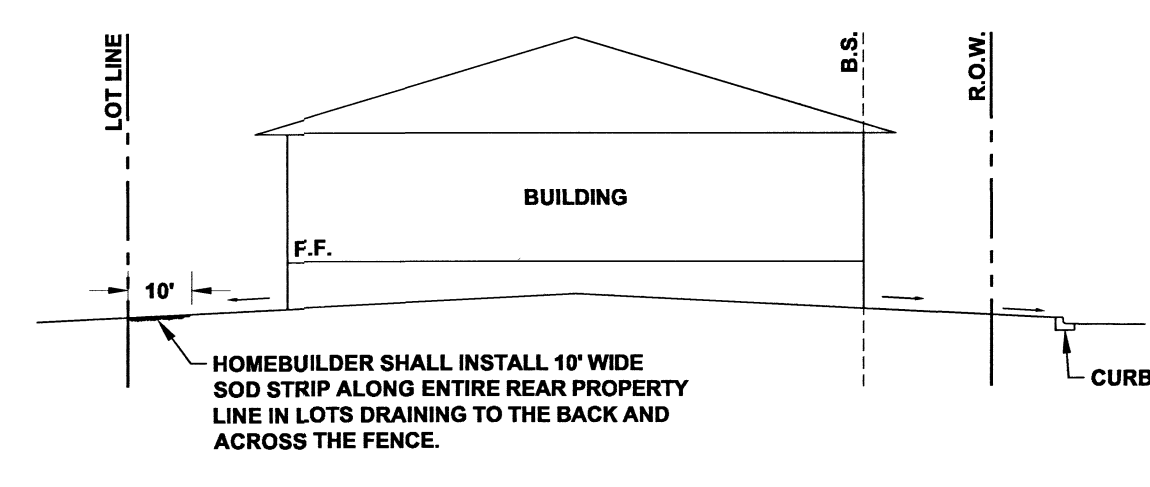
B TYPICAL "B" LOT GRADING SECTION SCALE: N.T.S.
