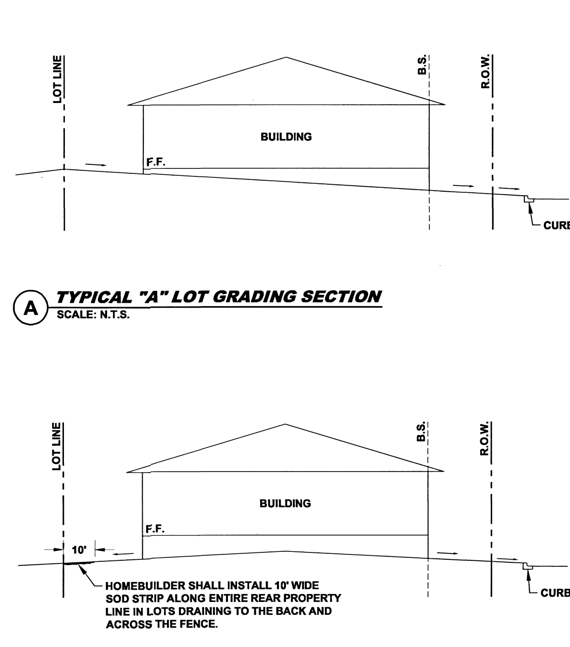
B TYPICAL "B" LOT GRADING SECTION SCALE: N.T.S.
