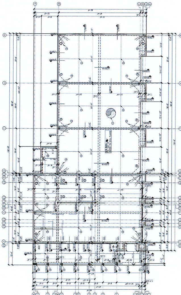
FOUNDATION PLAN SCALE: 1/8" = 1'-0"
