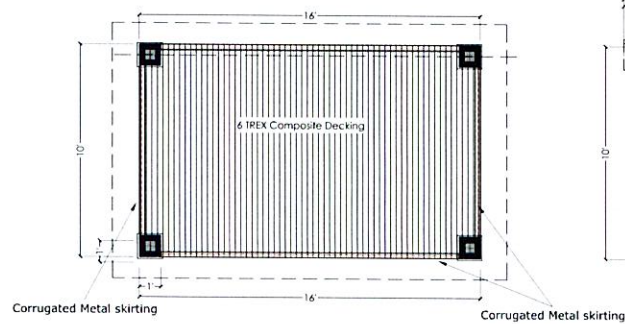
Plan view and Elevations 3/8" = 1'-0"
